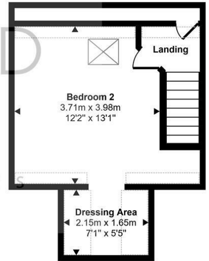
Second Floor Approx 24 sq m / 263 sq ft
